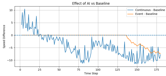
Fig. 12. Effect of AI vs Baseline. Continuous PSO (blue) corrects throughout; ET-PSO (orange) remains near-zero during safe phases and applies targeted correction only during risk phases.
